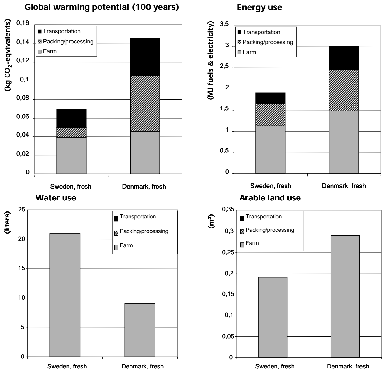
Figure 3.2. Environmental assessment of onion systems of different origins. Results are given per functional unit, i.e. per kg onions delivered to the gate of the wholesaler.
