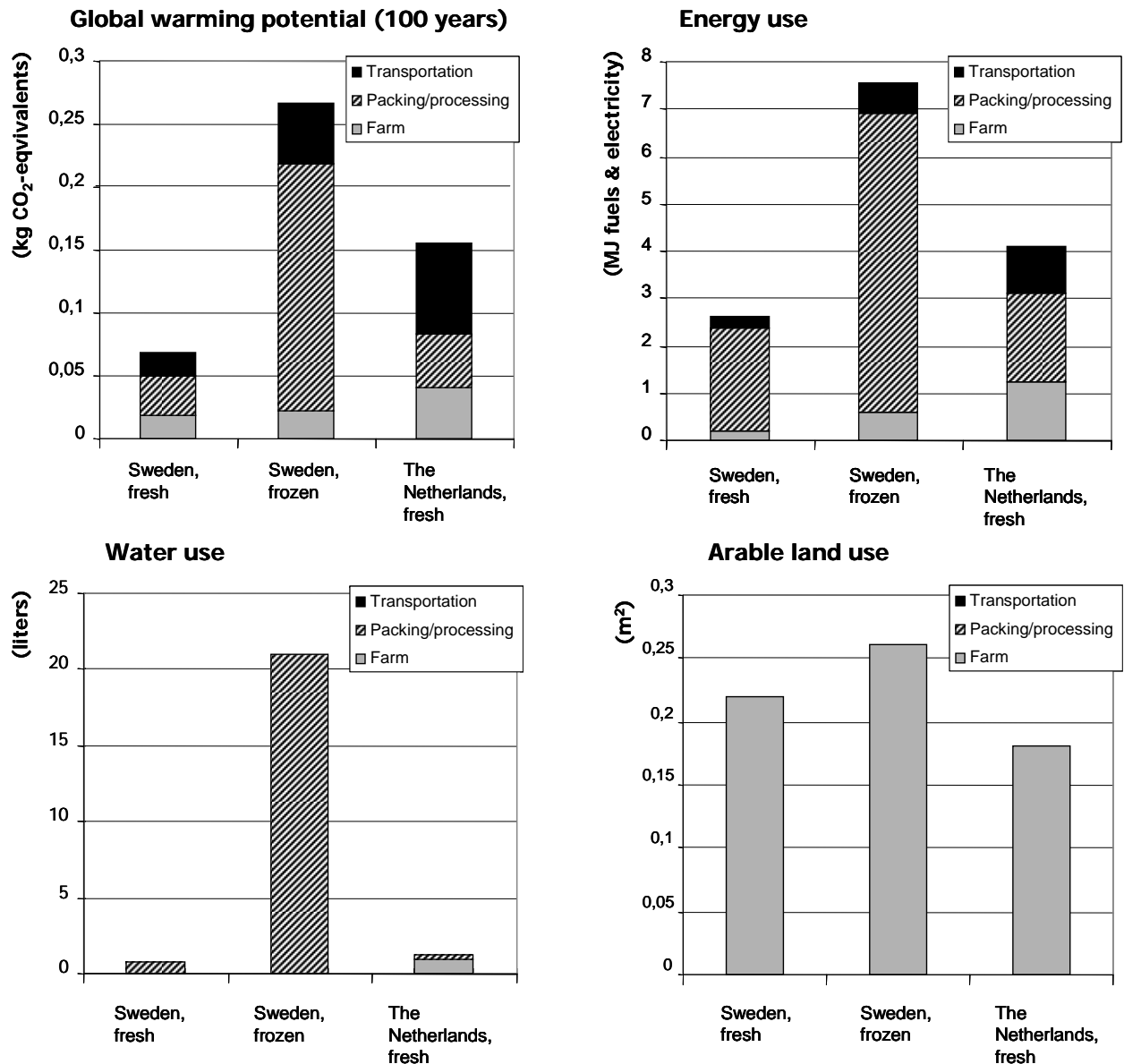
Figure 3.1. Environmental assessment of carrot systems of different origins and processing levels. Results are given per functional unit, i.e. per kg carrots delivered to the gate of the wholesaler.
